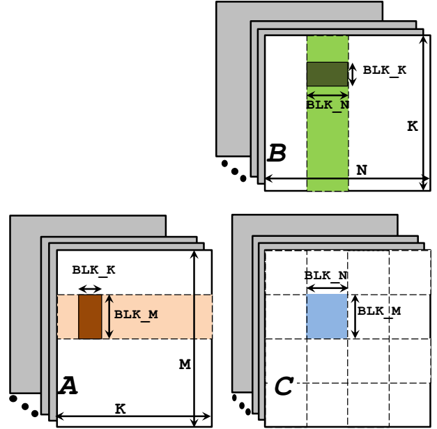
Fig. 1. Organization of the batched GEMM grid
