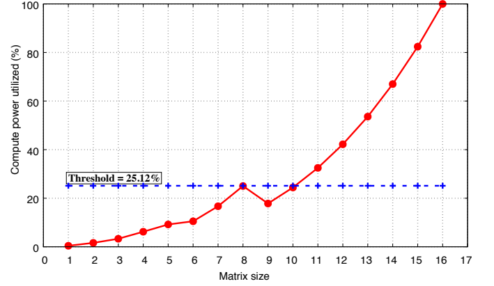
Fig. 14. The percentage of available Tensor Core compute power for square multiplications of small matrices.
