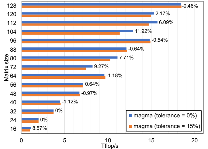
Fig. 6. Impact of the tolerance setting on the outcome of the tuning experiment. The performance is recorded for square sizes up to 128, with batchCount = 3,000 , on a Tesla V100 GPU.
