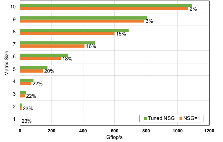
Fig. 8. Performance of the MAGMA kernel against different values of NSG . Results are shown for square sizes up to 10, with batchCount = 1M, on a Tesla V100 GPU.
