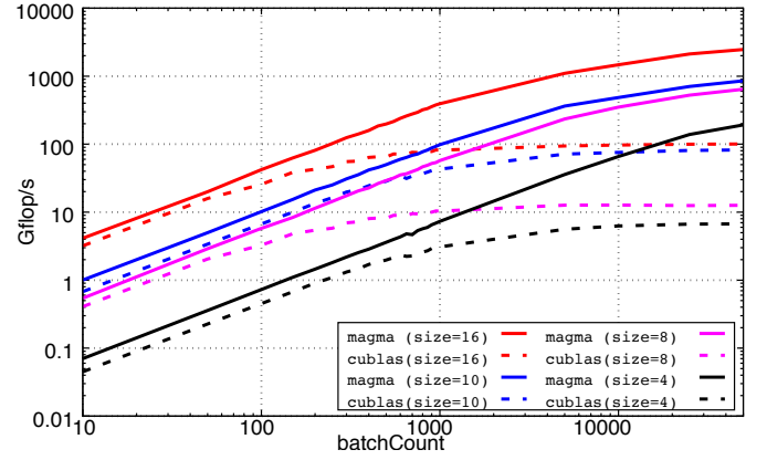
Fig. 17. Impact of \text{batchCount} on performance. Results are shown for very small selected sizes a Tesla V100 GPU
