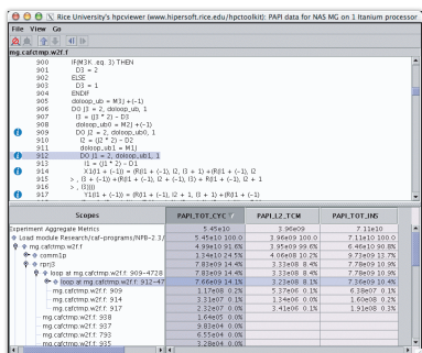
HPCView
