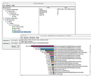
TAU
