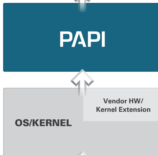
TAU
