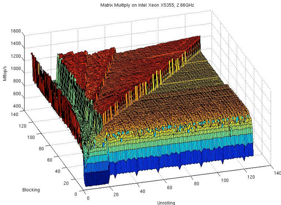
Figure 2. Example of parameter search space for auto-tuning.
